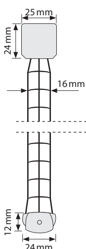
Standard Jalousie 16 mm Lamellen
